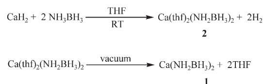
Scheme 1. Synthesis of 1 from calcium hydride and ammonia–borane.
